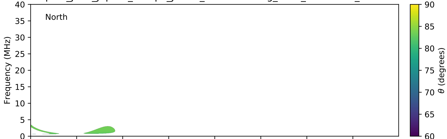
expres_juno_jupiter_europa_jrm09_lossc-wid1deg_3kev_20170616_v01.cdf
