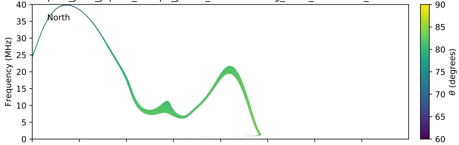
expres_juno_jupiter_europa_jrm09_lossc-wid1deg_3kev_20170612_v01.cdf
