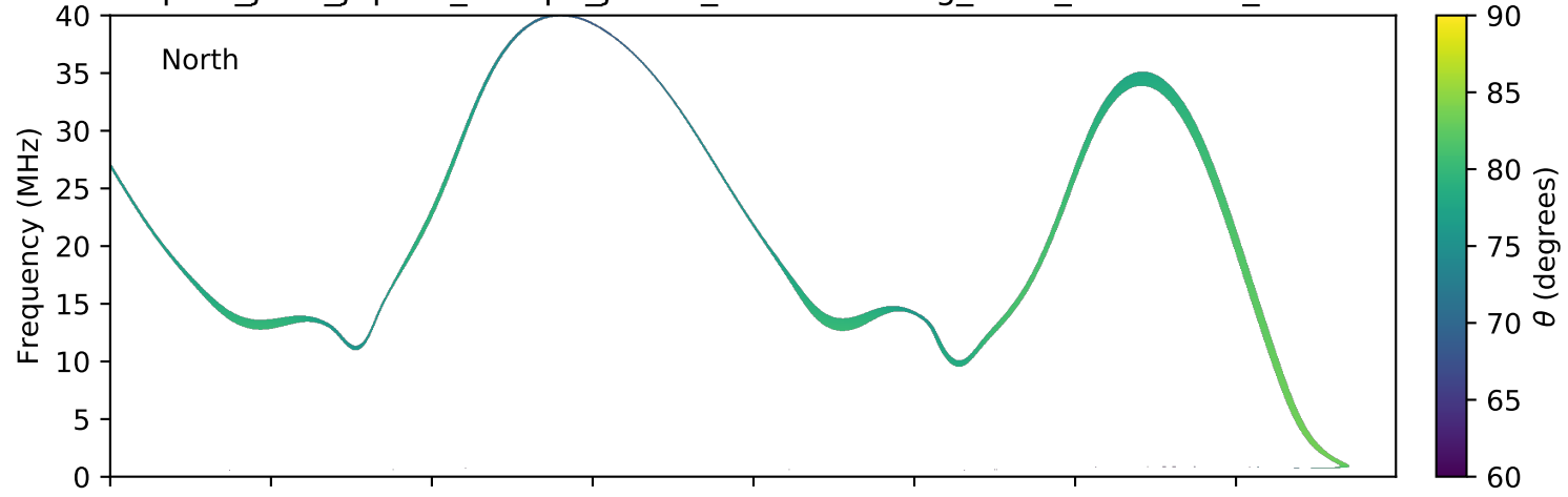
expres_juno_jupiter_europa_jrm09_lossc-wid1deg_3kev_20170608_v01.cdf
