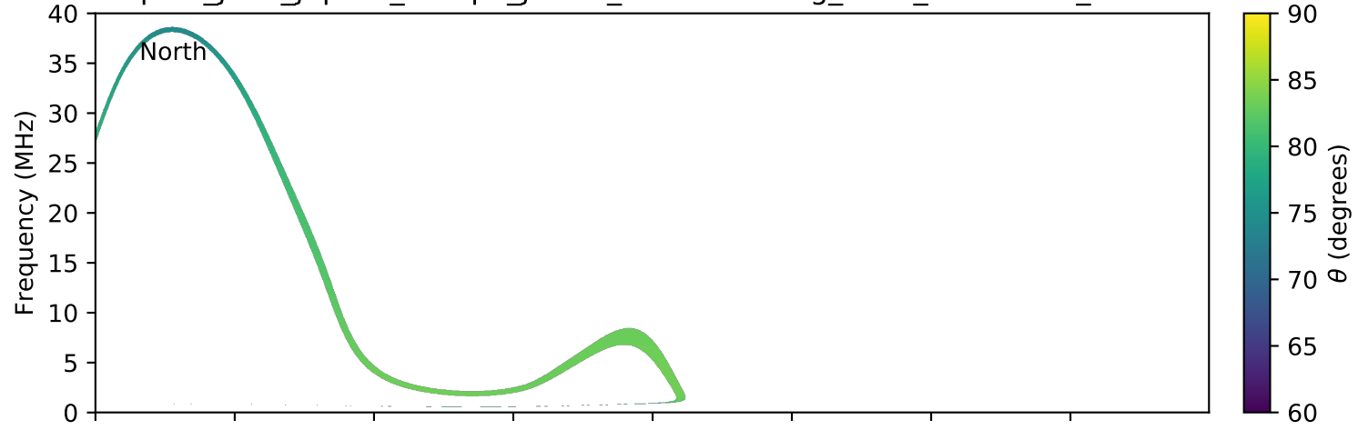
expres_juno_jupiter_europa_jrm09_lossc-wid1deg_3kev_20170605_v01.cdf
