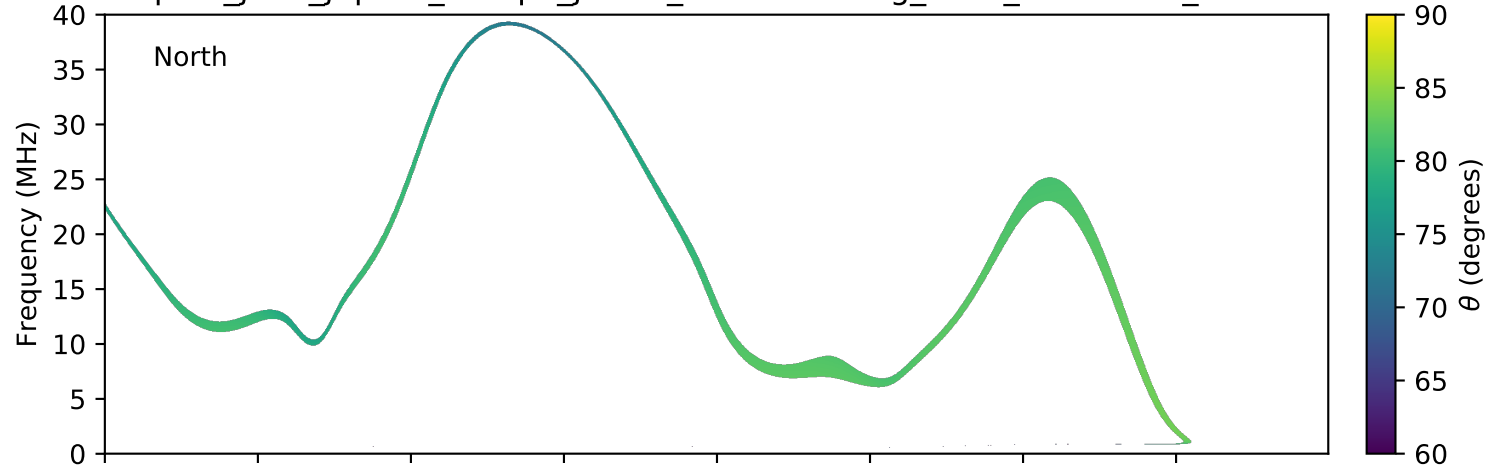
expres_juno_jupiter_europa_jrm09_lossc-wid1deg_3kev_20170601_v01.cdf
