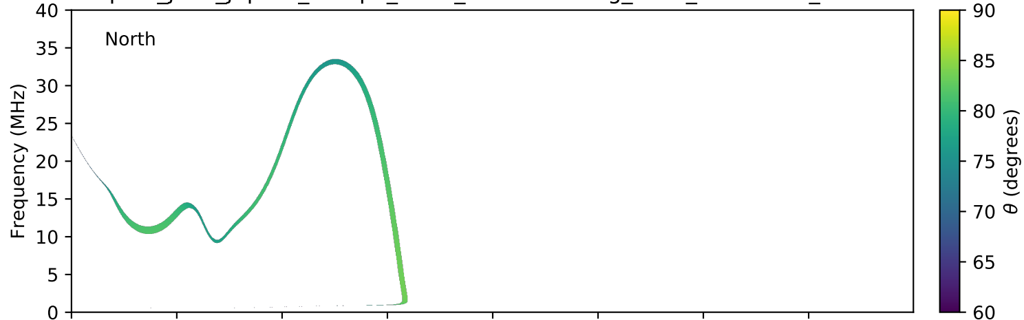
expres_juno_jupiter_europa_isaac_lossc-wid1deg_3kev_20170630_v01.cdf
