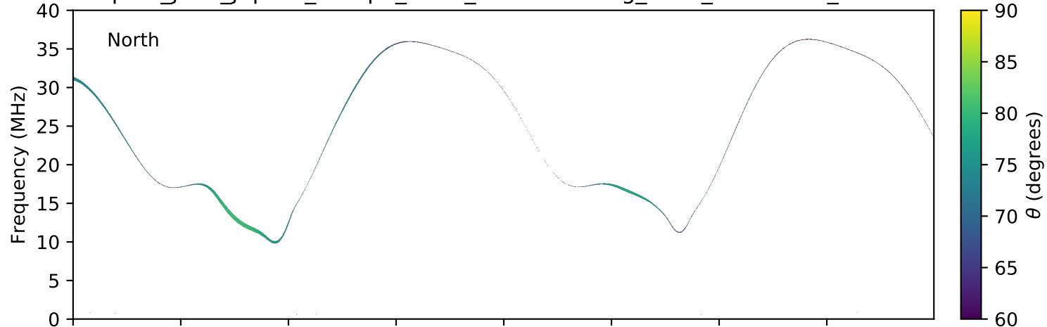
expres_juno_jupiter_europa_isaac_lossc-wid1deg_3kev_20170629_v01.cdf
