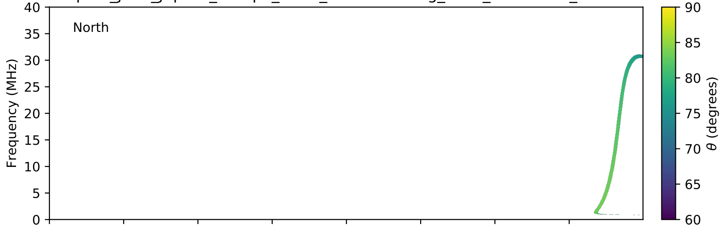
expres_juno_jupiter_europa_isaac_lossc-wid1deg_3kev_20170628_v01.cdf
