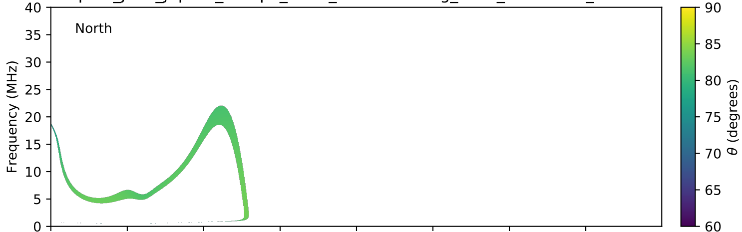
expres_juno_jupiter_europa_isaac_lossc-wid1deg_3kev_20170623_v01.cdf
