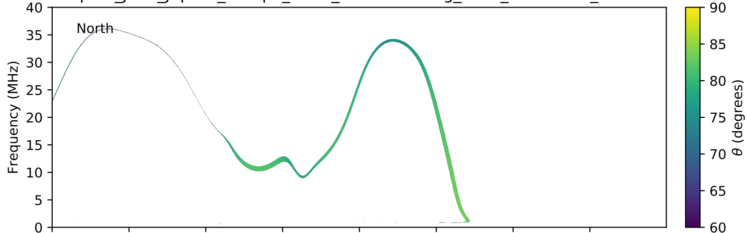
expres_juno_jupiter_europa_isaac_lossc-wid1deg_3kev_20170619_v01.cdf
