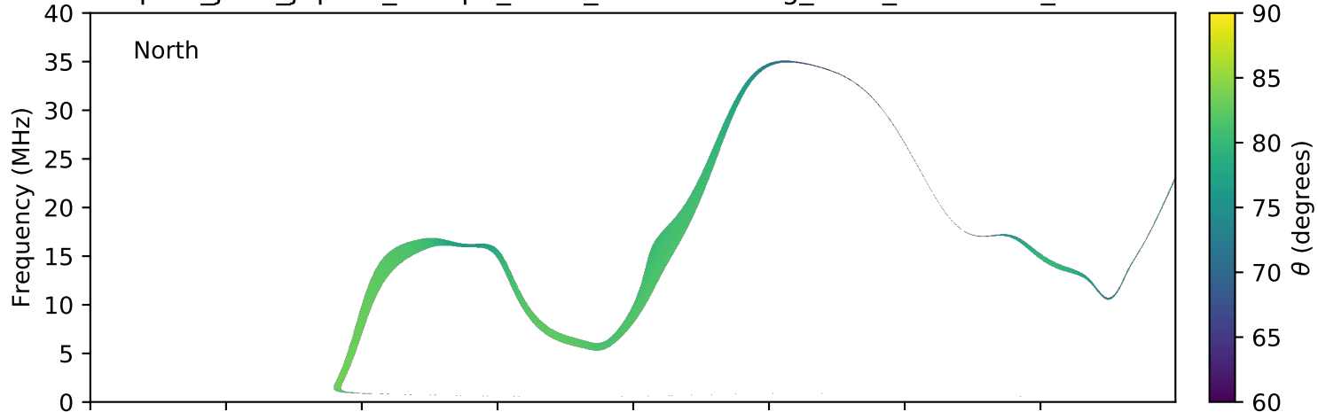
expres_juno_jupiter_europa_isaac_lossc-wid1deg_3kev_20170618_v01.cdf
