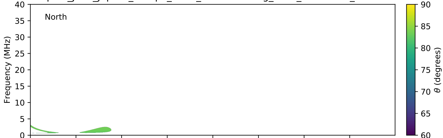
expres_juno_jupiter_europa_isaac_lossc-wid1deg_3kev_20170616_v01.cdf
