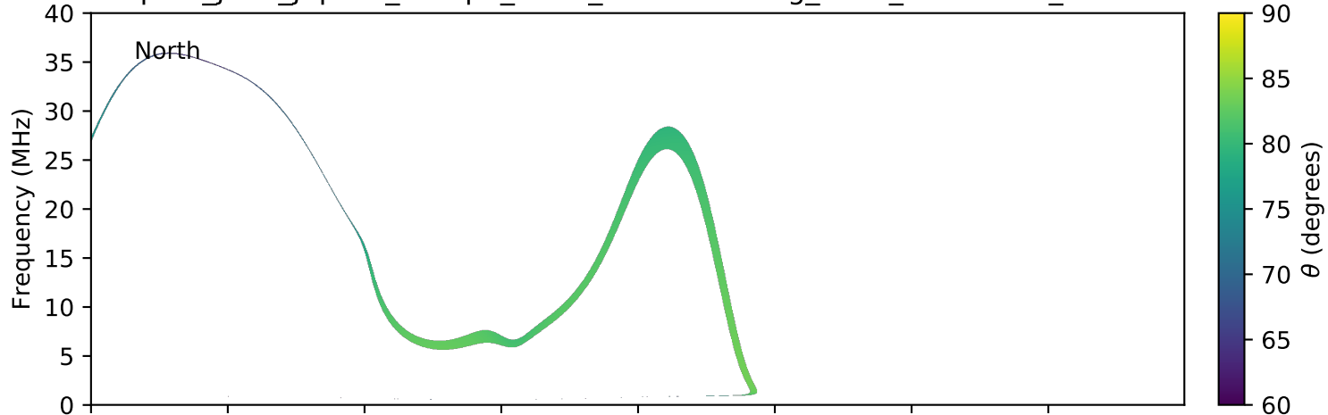
expres_juno_jupiter_europa_isaac_lossc-wid1deg_3kev_20170612_v01.cdf
