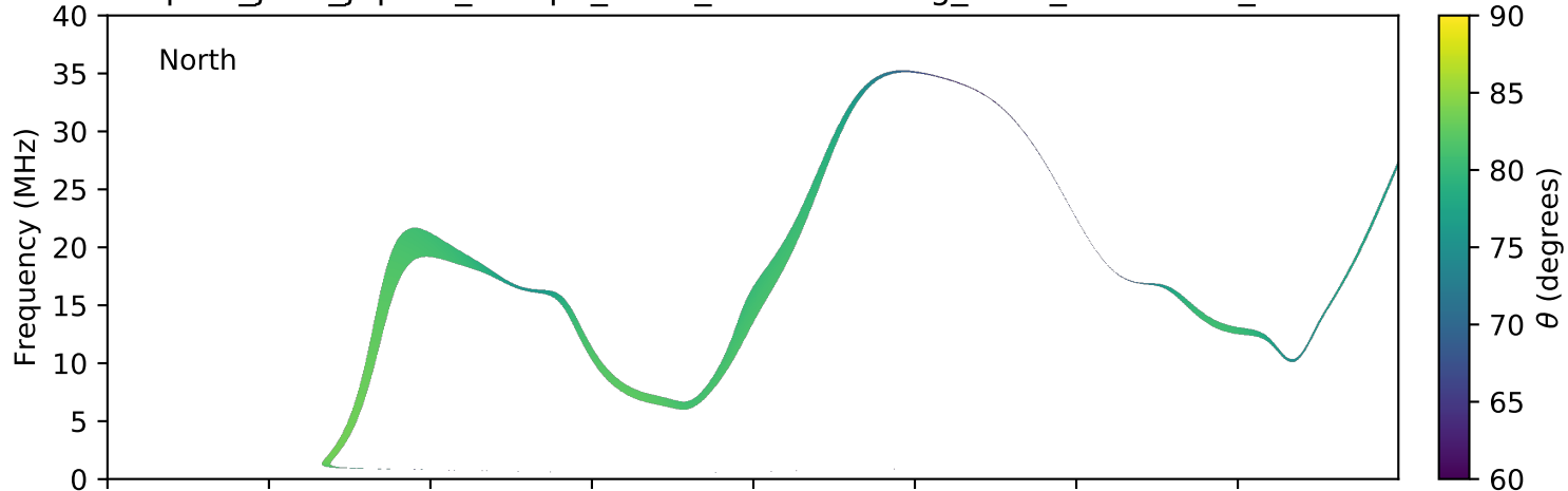
expres_juno_jupiter_europa_isaac_lossc-wid1deg_3kev_20170611_v01.cdf
