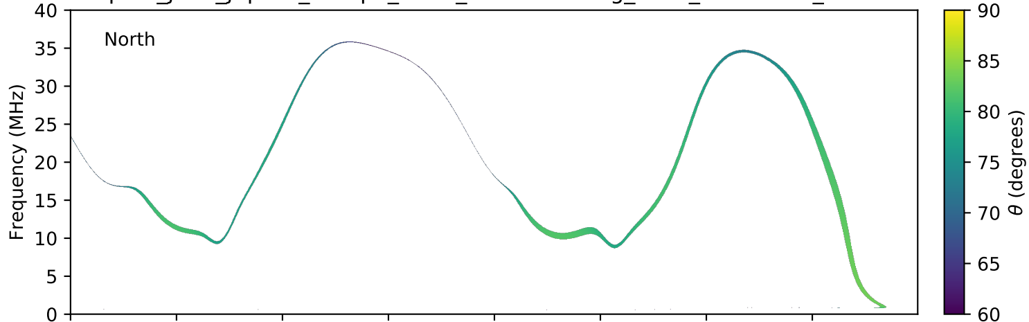
expres_juno_jupiter_europa_isaac_lossc-wid1deg_3kev_20170608_v01.cdf
