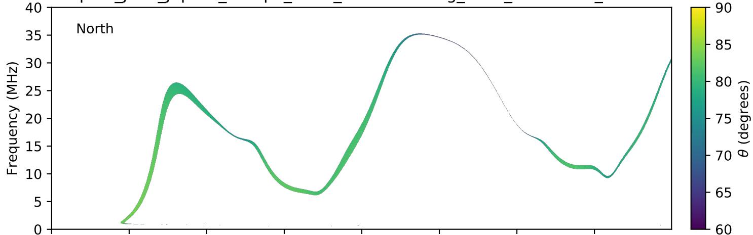
expres_juno_jupiter_europa_isaac_lossc-wid1deg_3kev_20170604_v01.cdf
