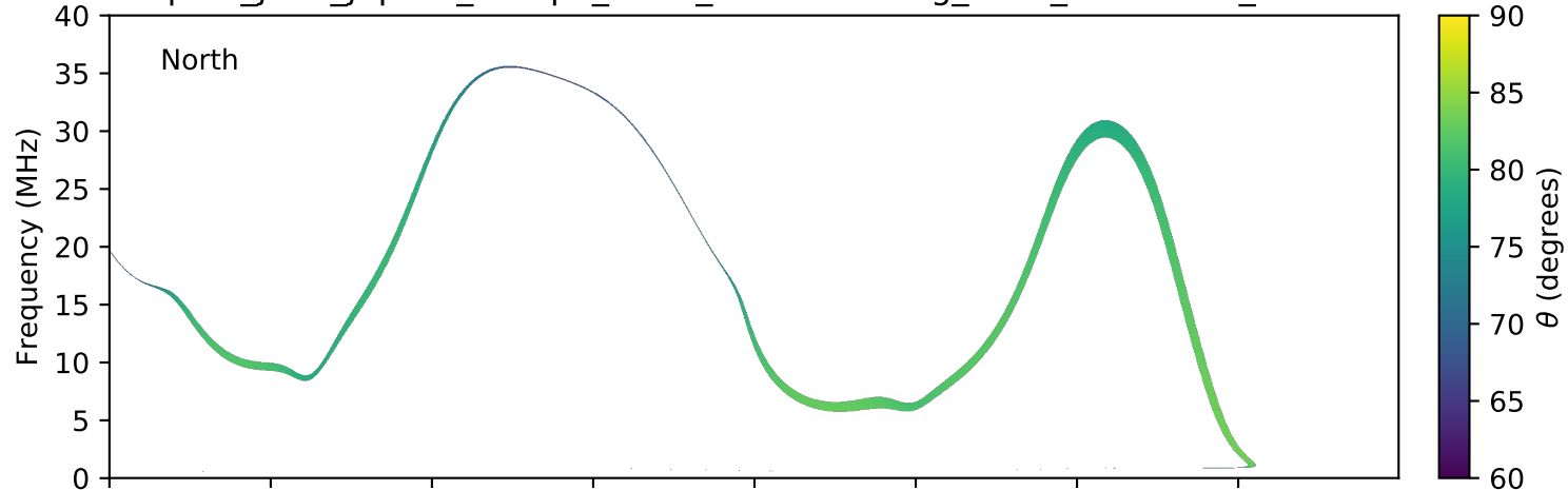
expres_juno_jupiter_europa_isaac_lossc-wid1deg_3kev_20170601_v01.cdf
