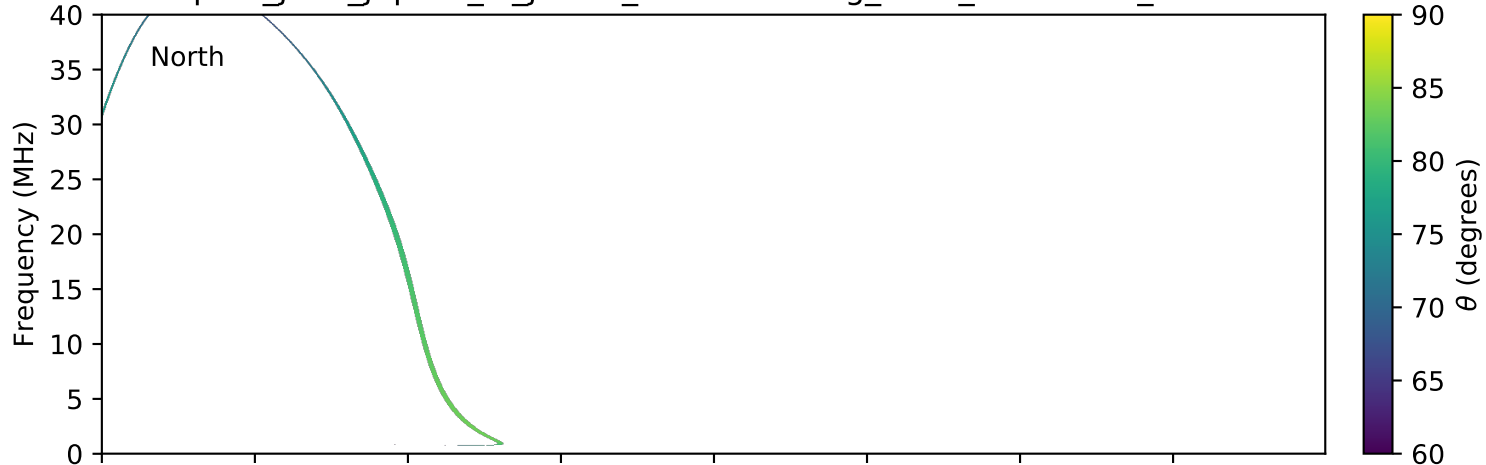
expres_juno_jupiter_io_jrm09_lossc-wid1deg_3kev_20170531_v01.cdf
