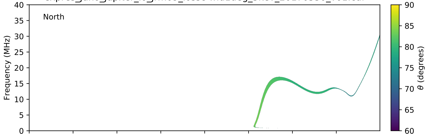
expres_juno_jupiter_io_jrm09_lossc-wid1deg_3kev_20170530_v01.cdf
