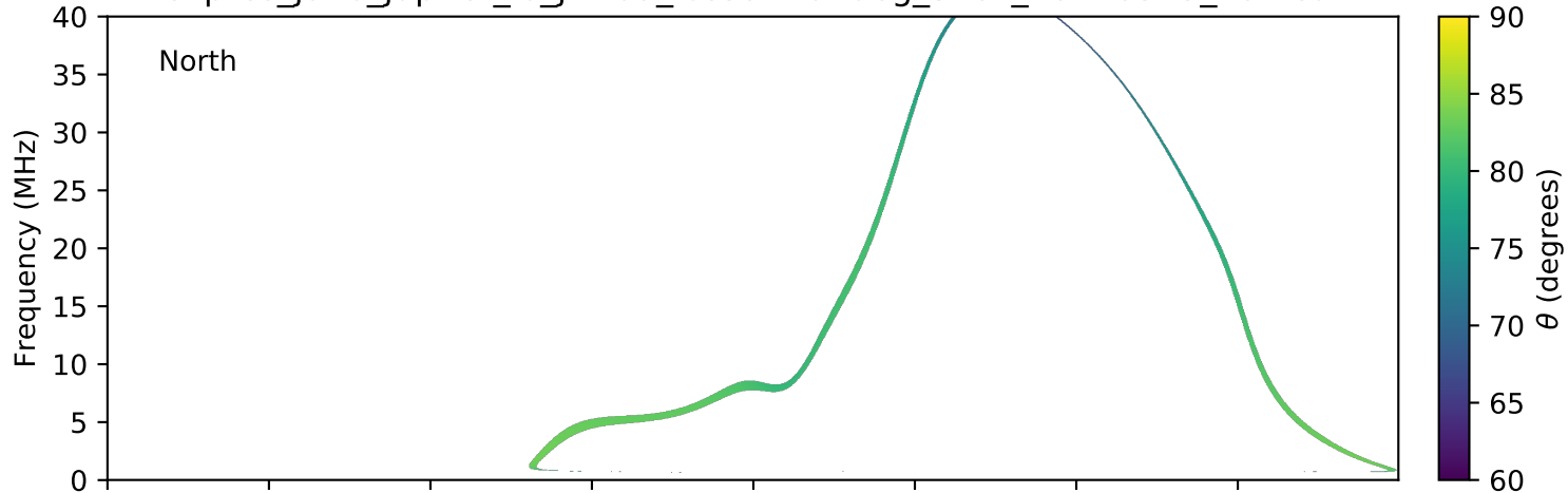
expres_juno_jupiter_io_jrm09_lossc-wid1deg_3kev_20170525_v01.cdf
