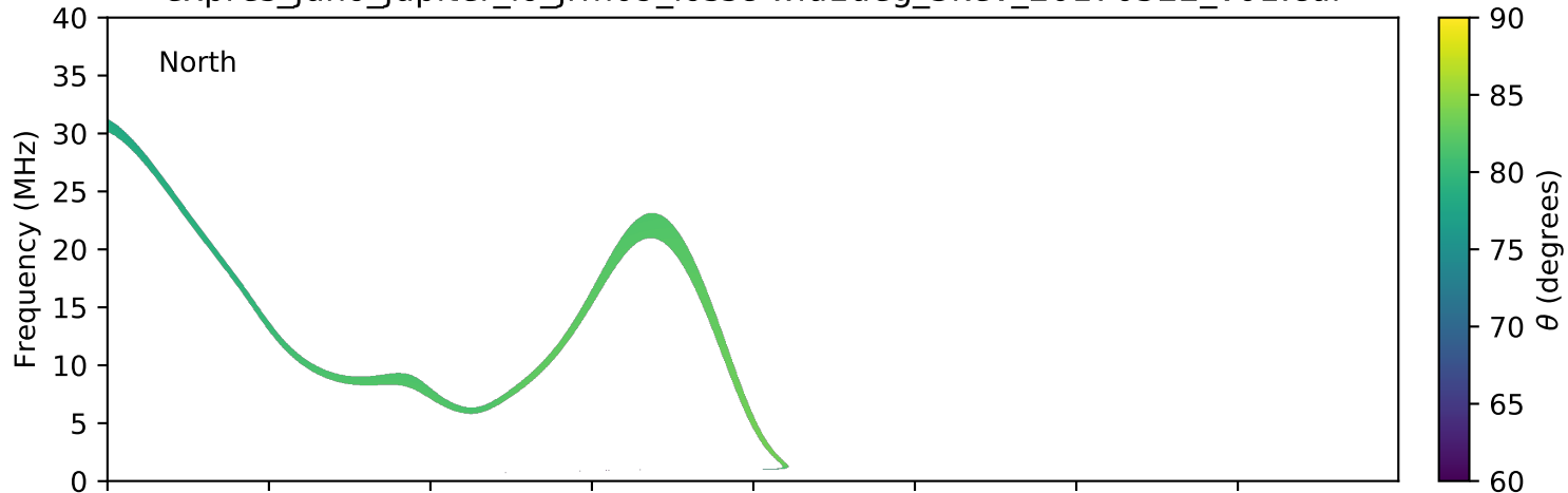
expres_juno_jupiter_io_jrm09_lossc-wid1deg_3kev_20170522_v01.cdf
