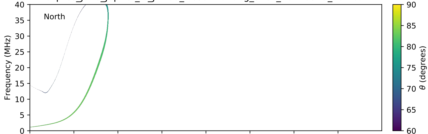
expres_juno_jupiter_io_jrm09_lossc-wid1deg_3kev_20170519_v01.cdf
