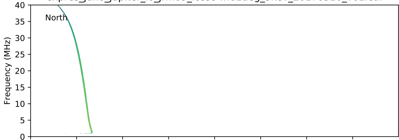
expres_juno_jupiter_io_jrm09_lossc-wid1deg_3kev_20170510_v01.cdf
