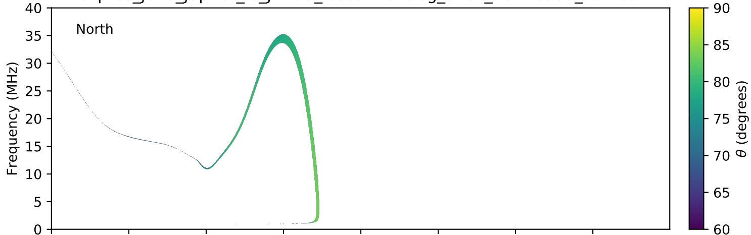
expres_juno_jupiter_io_jrm09_lossc-wid1deg_3kev_20170508_v01.cdf
