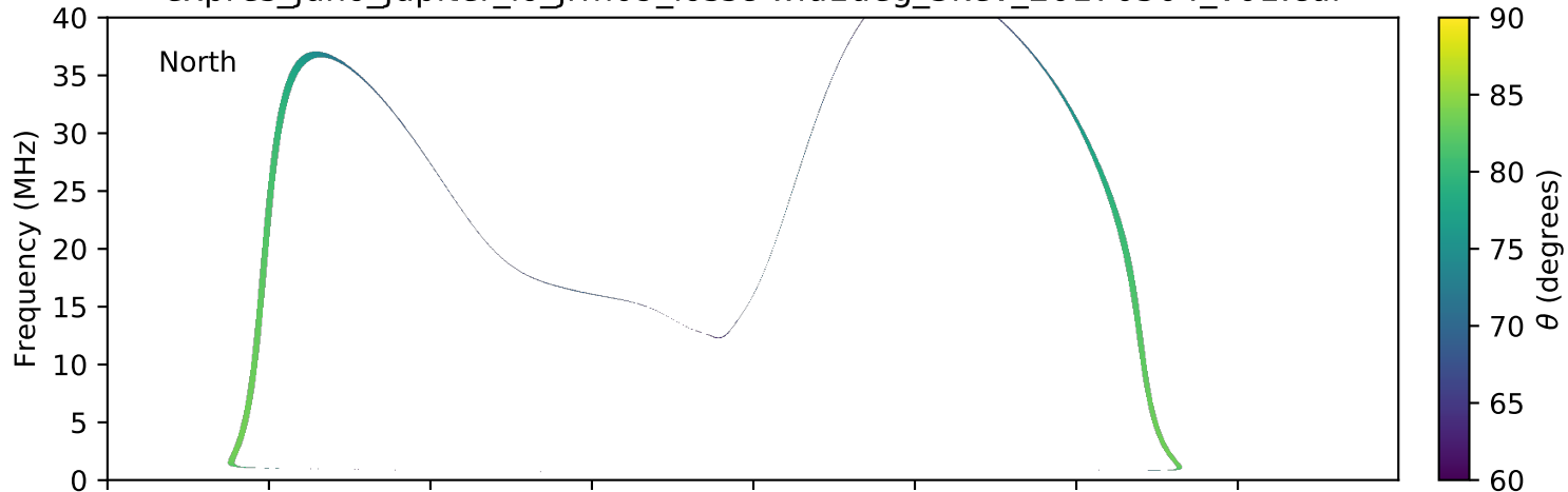
expres_juno_jupiter_io_jrm09_lossc-wid1deg_3kev_20170504_v01.cdf
