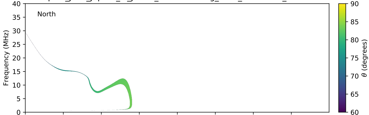
expres_juno_jupiter_io_jrm09_lossc-wid1deg_3kev_20170501_v01.cdf
