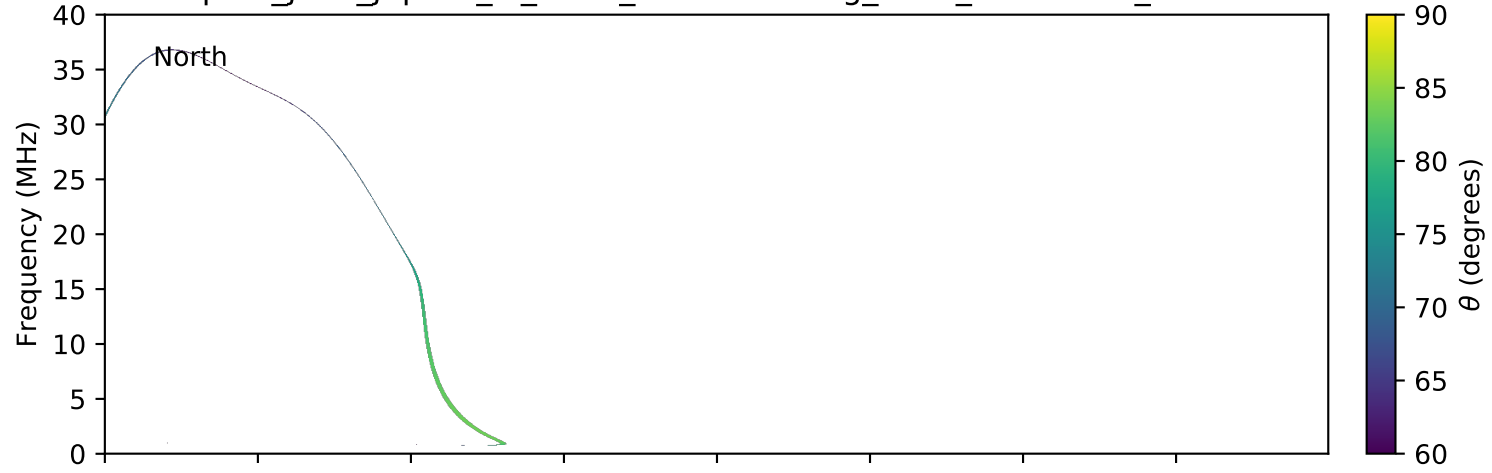
expres_juno_jupiter_io_isaac_lossc-wid1deg_3kev_20170531_v01.cdf
