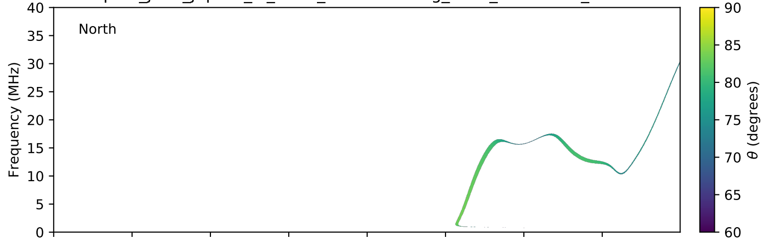
expres_juno_jupiter_io_isaac_lossc-wid1deg_3kev_20170530_v01.cdf
