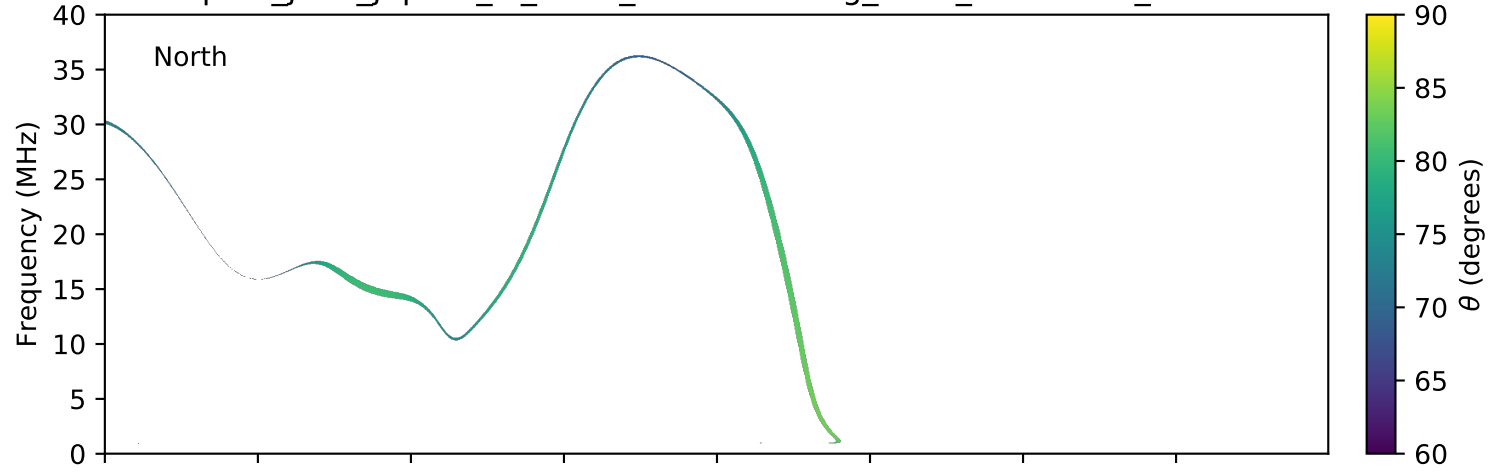
expres_juno_jupiter_io_isaac_lossc-wid1deg_3kev_20170529_v01.cdf
