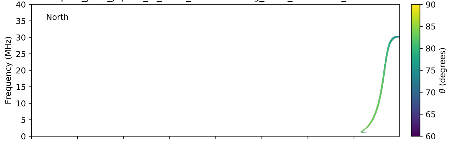
expres_juno_jupiter_io_isaac_lossc-wid1deg_3kev_20170528_v01.cdf
