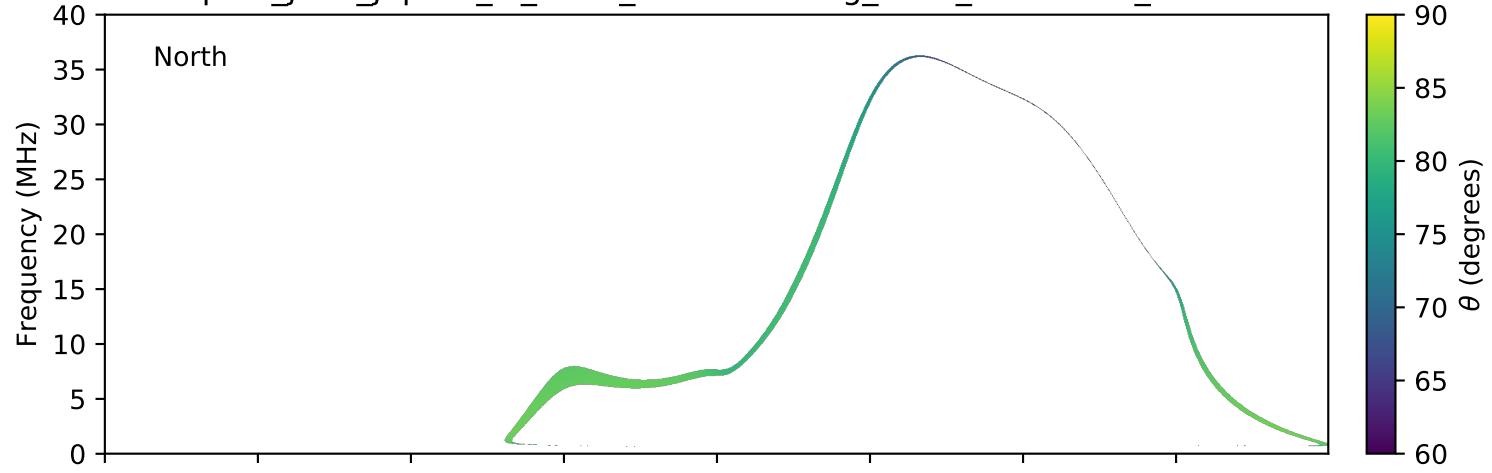
expres_juno_jupiter_io_isaac_lossc-wid1deg_3kev_20170525_v01.cdf
