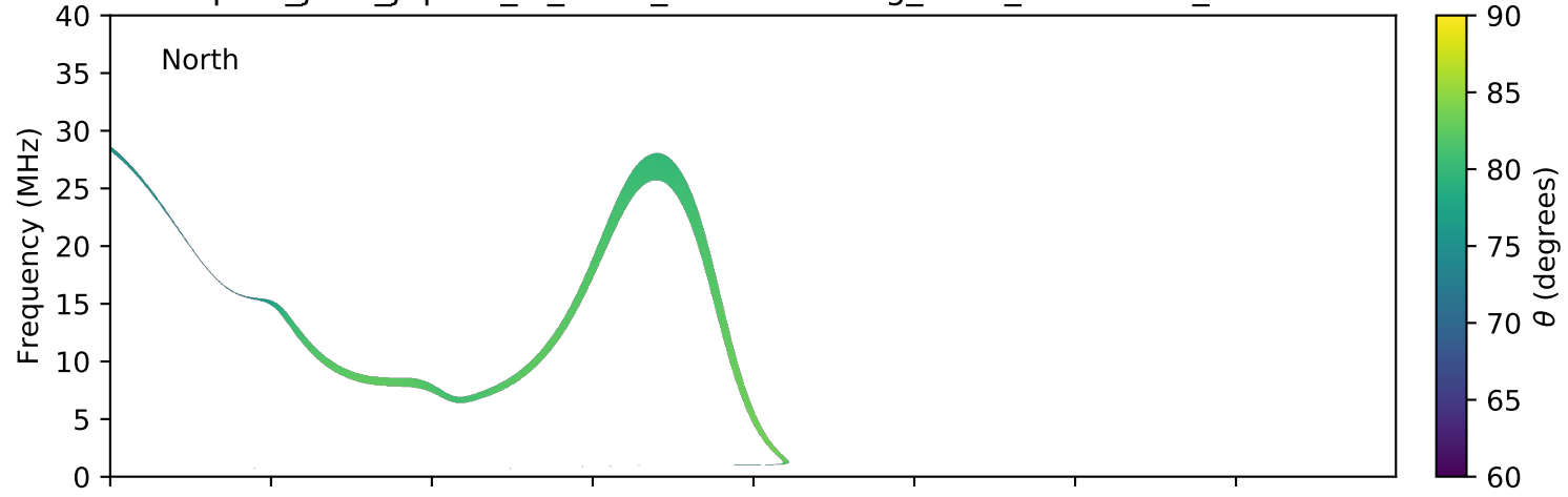
expres_juno_jupiter_io_isaac_lossc-wid1deg_3kev_20170522_v01.cdf
