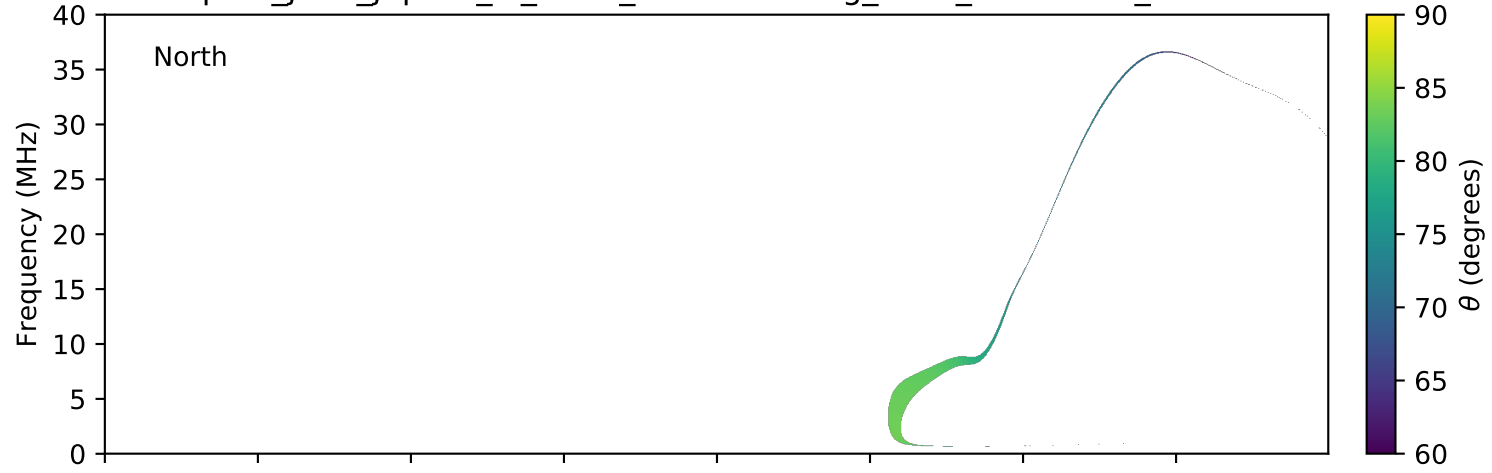
expres_juno_jupiter_io_isaac_lossc-wid1deg_3kev_20170514_v01.cdf
