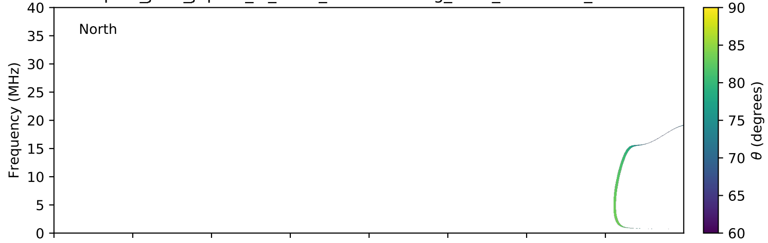
expres_juno_jupiter_io_isaac_lossc-wid1deg_3kev_20170512_v01.cdf
