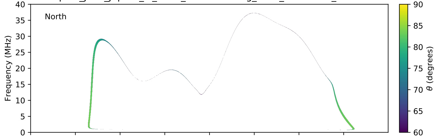
expres_juno_jupiter_io_isaac_lossc-wid1deg_3kev_20170511_v01.cdf
