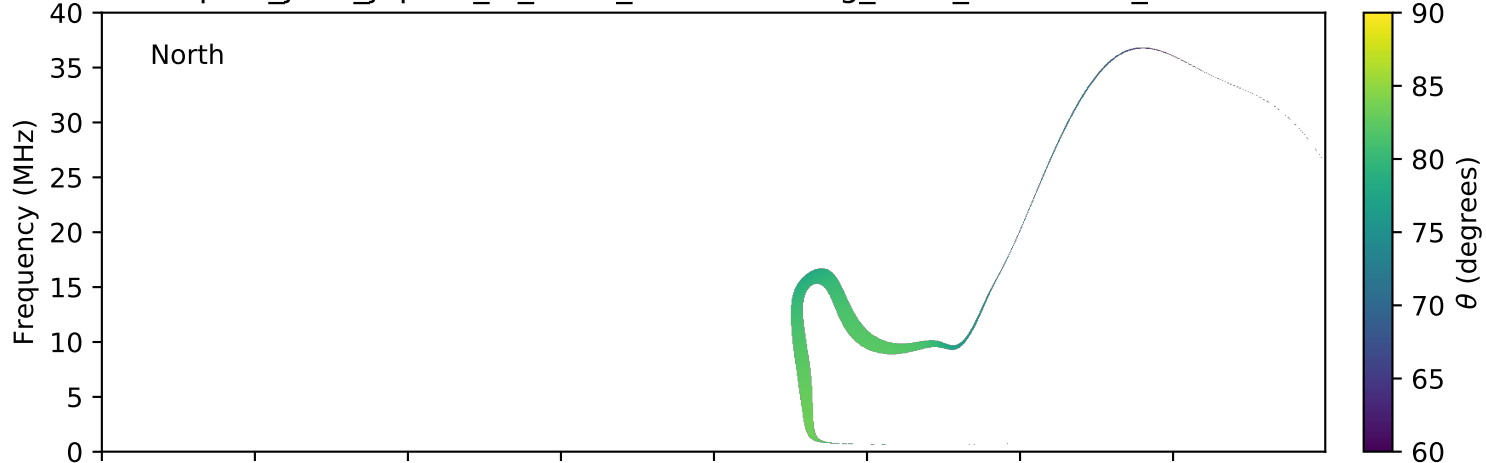
expres_juno_jupiter_io_isaac_lossc-wid1deg_3kev_20170507_v01.cdf
