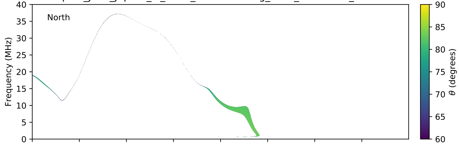
expres_juno_jupiter_io_isaac_lossc-wid1deg_3kev_20170506_v01.cdf
