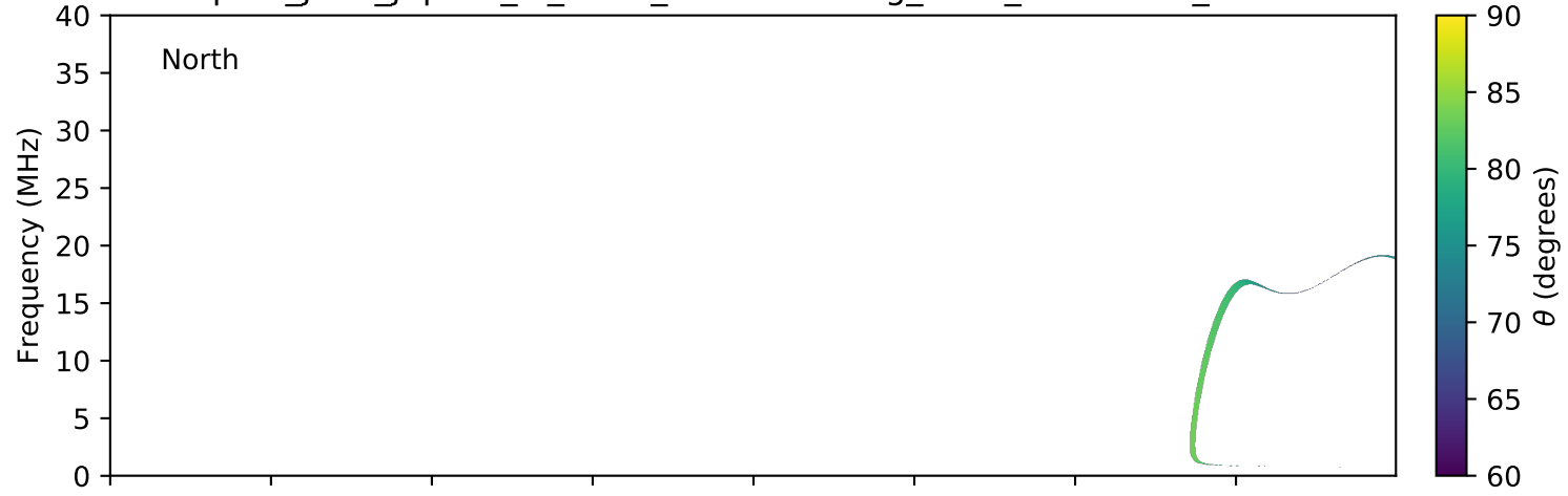
expres_juno_jupiter_io_isaac_lossc-wid1deg_3kev_20170505_v01.cdf
