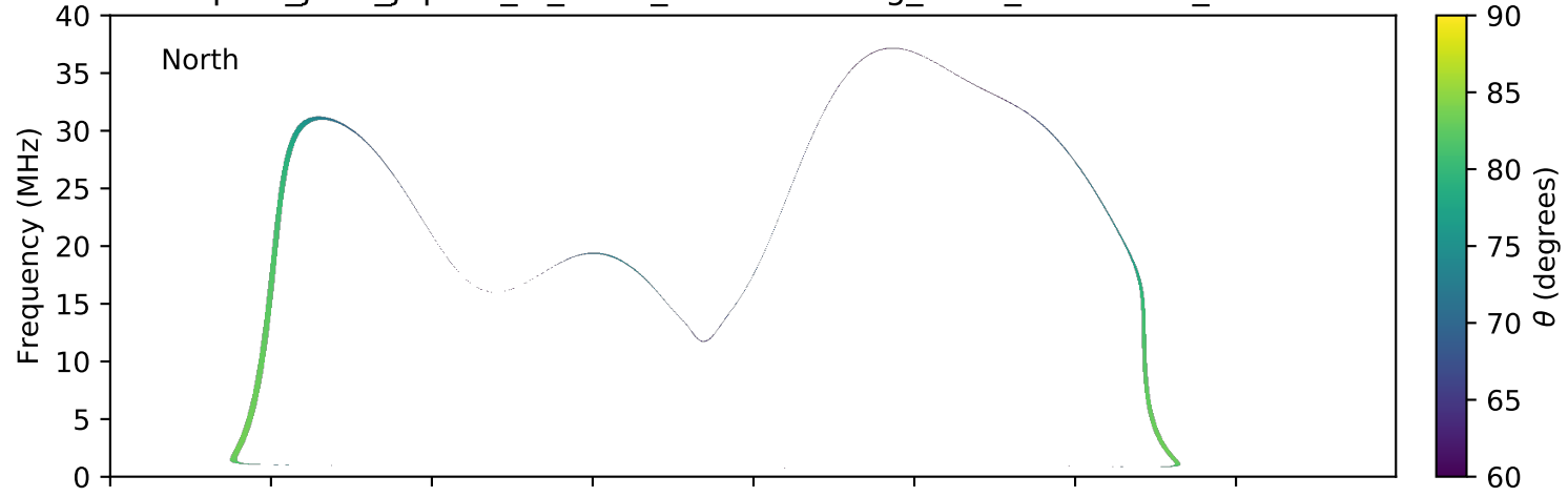
expres_juno_jupiter_io_isaac_lossc-wid1deg_3kev_20170504_v01.cdf
