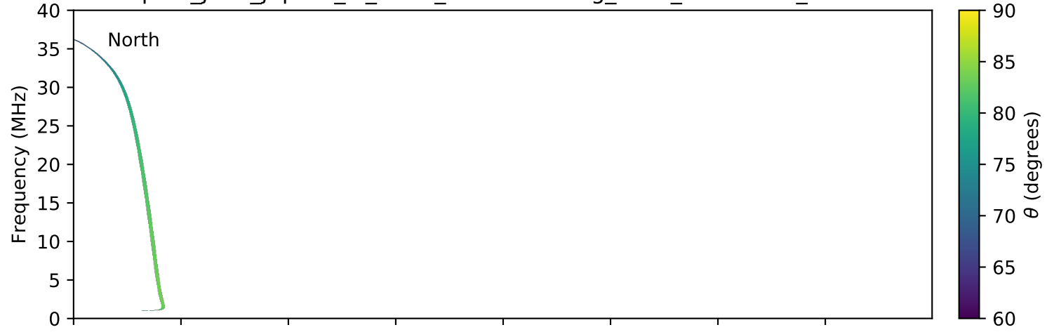
expres_juno_jupiter_io_isaac_lossc-wid1deg_3kev_20170503_v01.cdf
