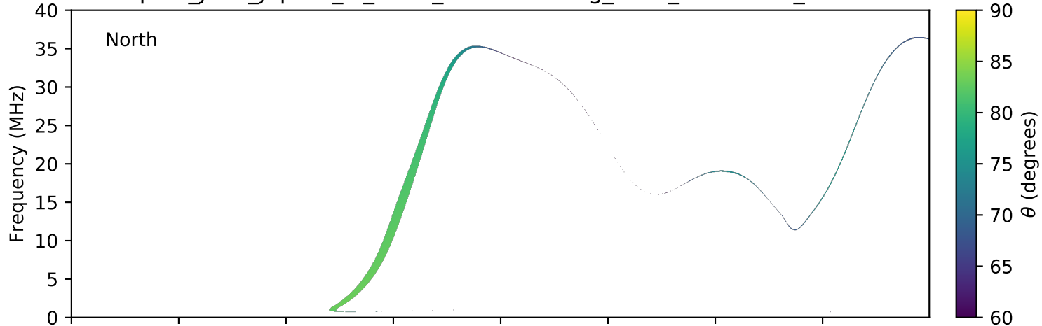
expres_juno_jupiter_io_isaac_lossc-wid1deg_3kev_20170502_v01.cdf
