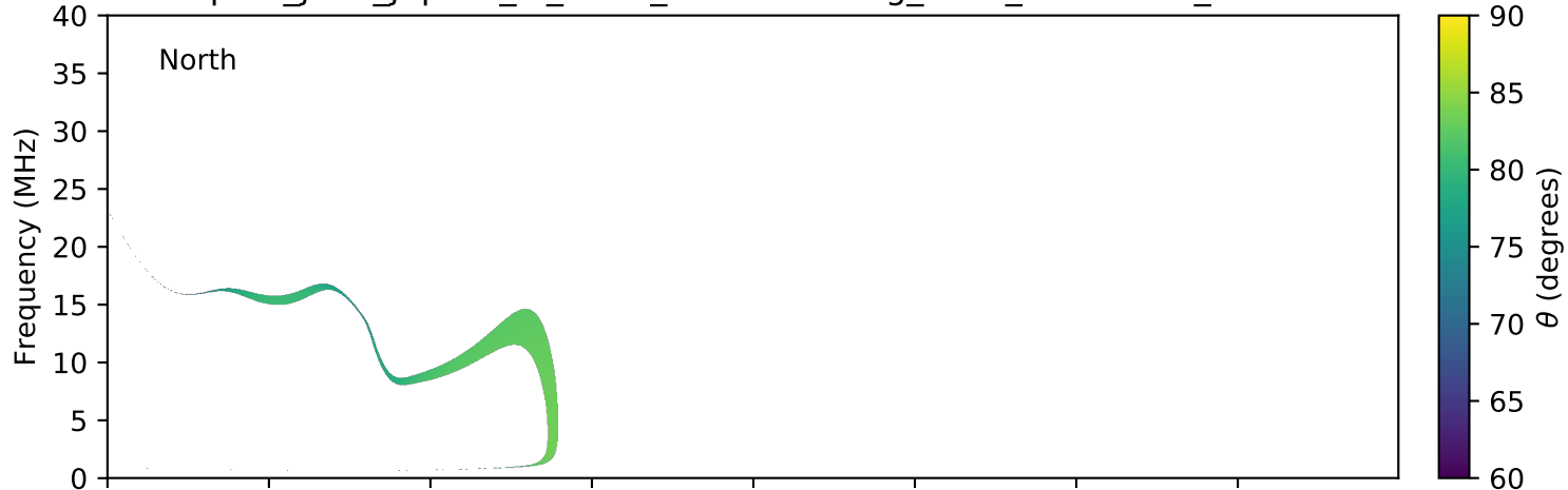
expres_juno_jupiter_io_isaac_lossc-wid1deg_3kev_20170501_v01.cdf
