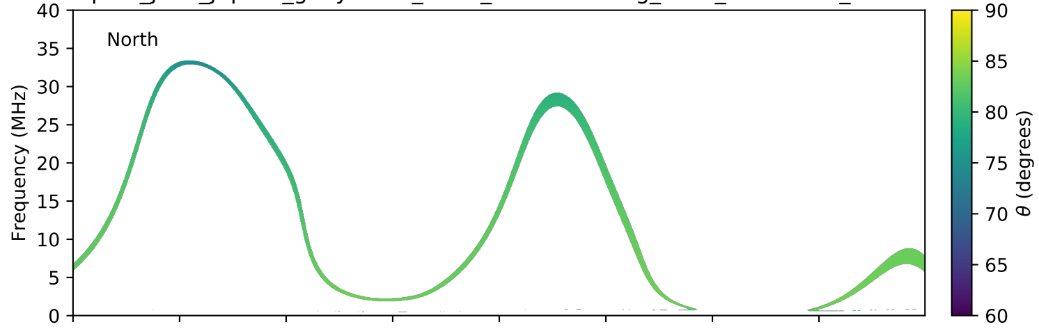
expres_juno_jupiter_ganymede_isaac_lossc-wid1deg_3kev_20170526_v01.cdf
