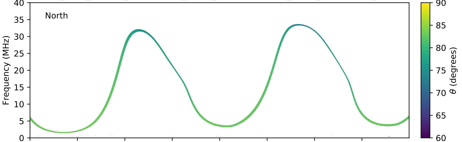
expres_juno_jupiter_ganymede_isaac_lossc-wid1deg_3kev_20170525_v01.cdf
