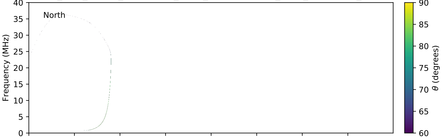
expres_juno_jupiter_ganymede_isaac_lossc-wid1deg_3kev_20170519_v01.cdf
