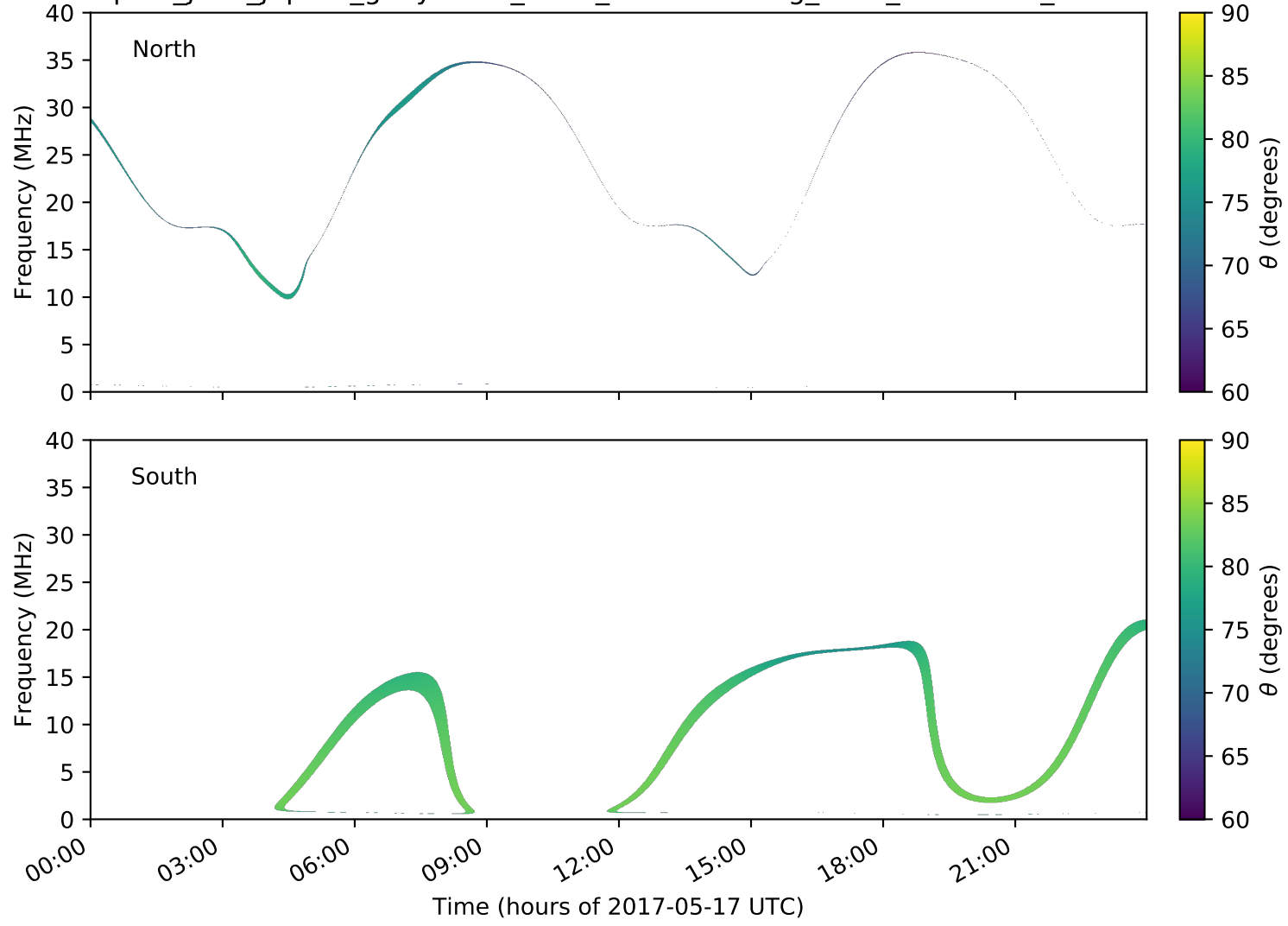
expres_juno_jupiter_ganymede_isaac_lossc-wid1deg_3kev_20170517_v01.cdf
