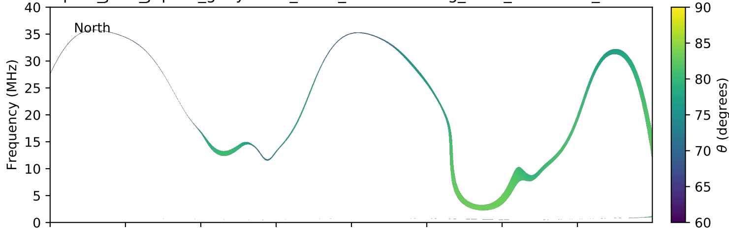
expres_juno_jupiter_ganymede_isaac_lossc-wid1deg_3kev_20170512_v01.cdf
