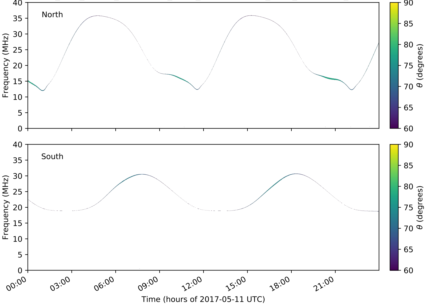
expres_juno_jupiter_ganymede_isaac_lossc-wid1deg_3kev_20170511_v01.cdf
