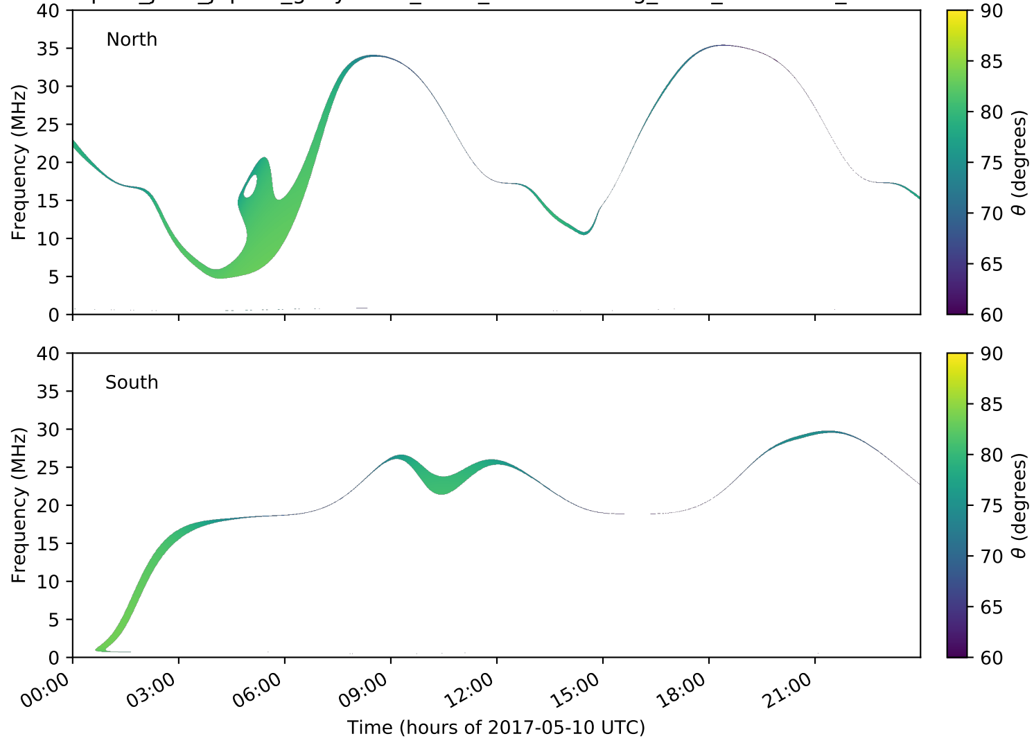
expres_juno_jupiter_ganymede_isaac_lossc-wid1deg_3kev_20170510_v01.cdf
