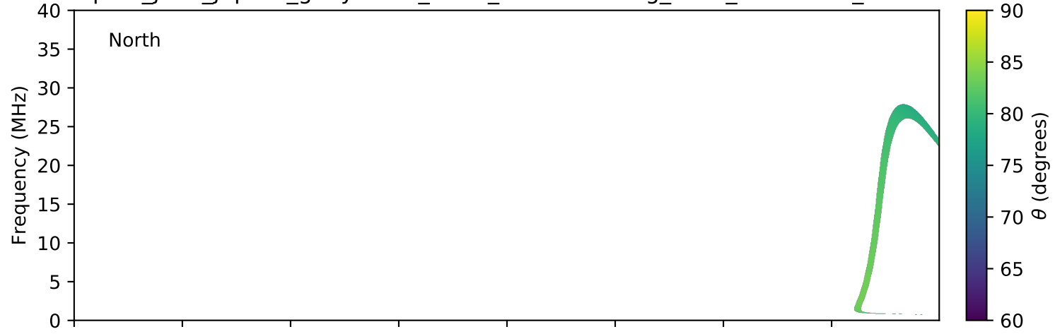
expres_juno_jupiter_ganymede_isaac_lossc-wid1deg_3kev_20170509_v01.cdf
